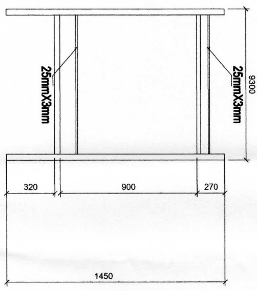
03 ELEVATION SCALE 1:100
